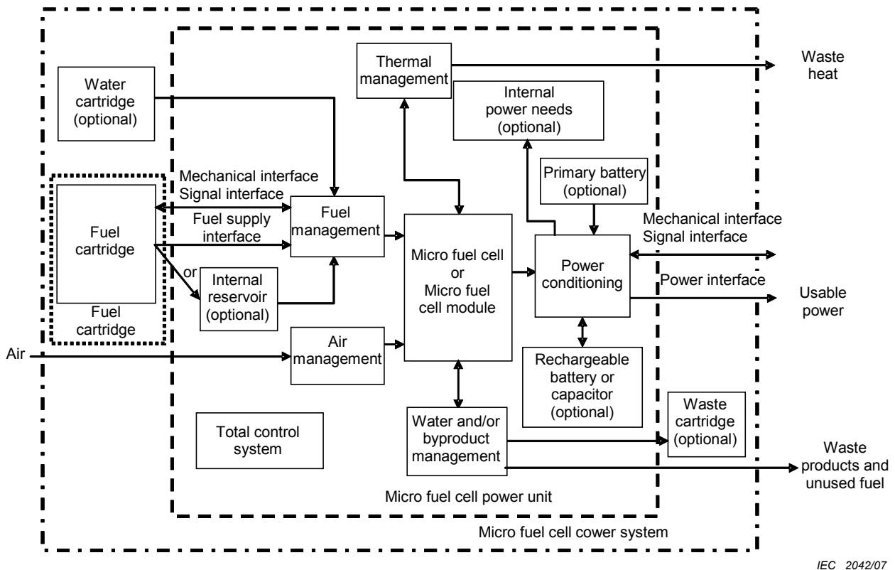
Figure 1 – Functional arrangement addressed in the scope of this standard
