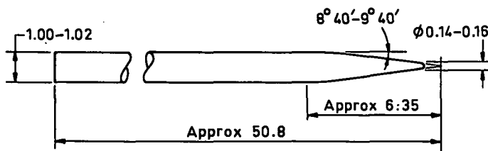
Fig. 1. NEEDLE FOR PENETRATION TEST
